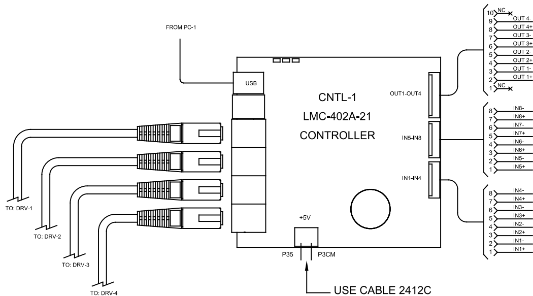
LUMINARY CONTROLLER
